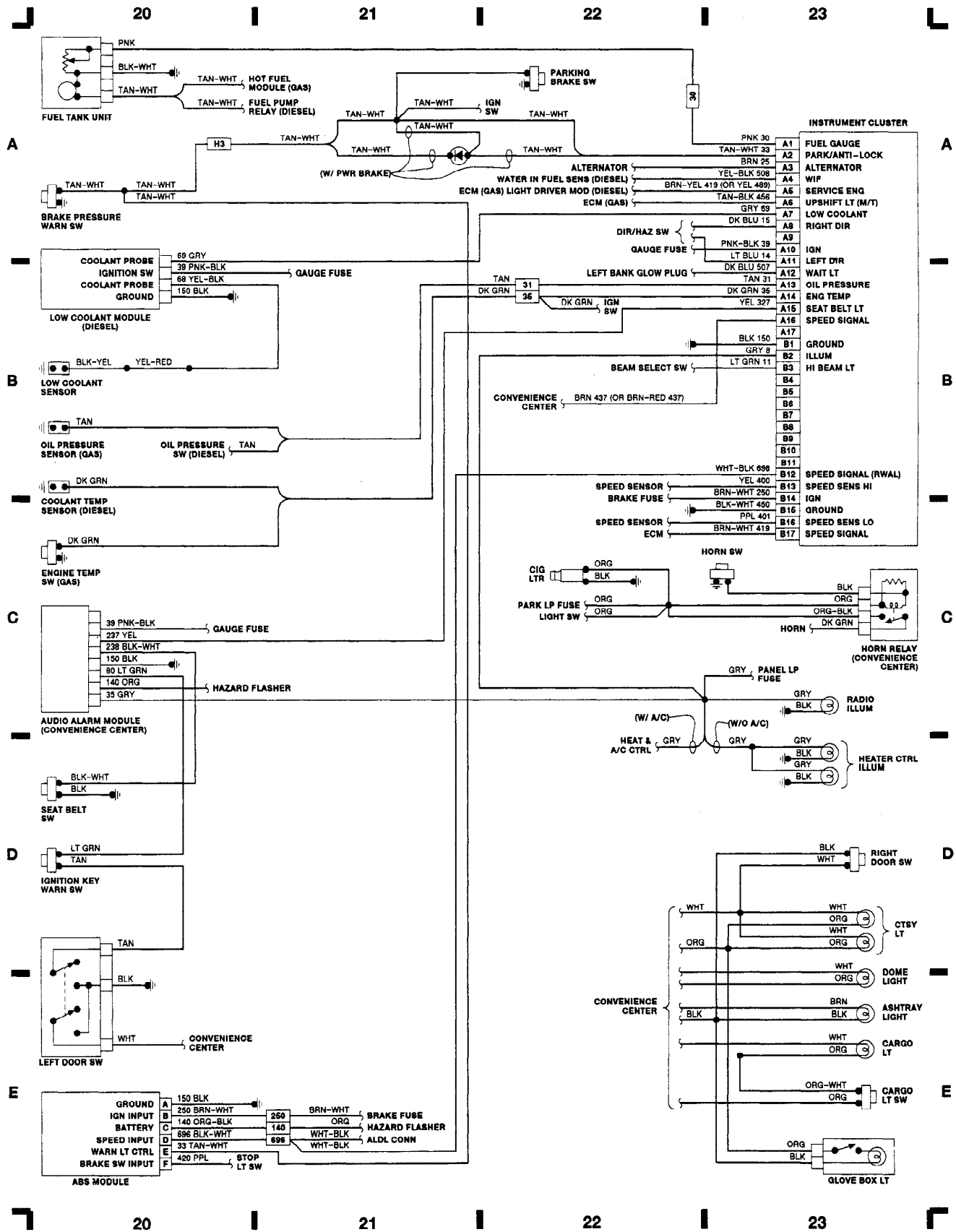
Fig. 6: Instrument Cluster 1990 Chevrolet Pickup K1500
