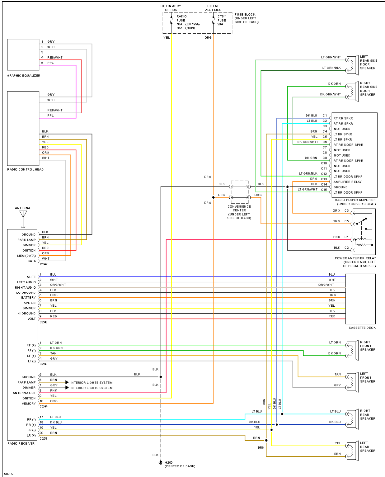
Fig. 94: AM/FM Stereo, W/ Cassette & Amplifier
