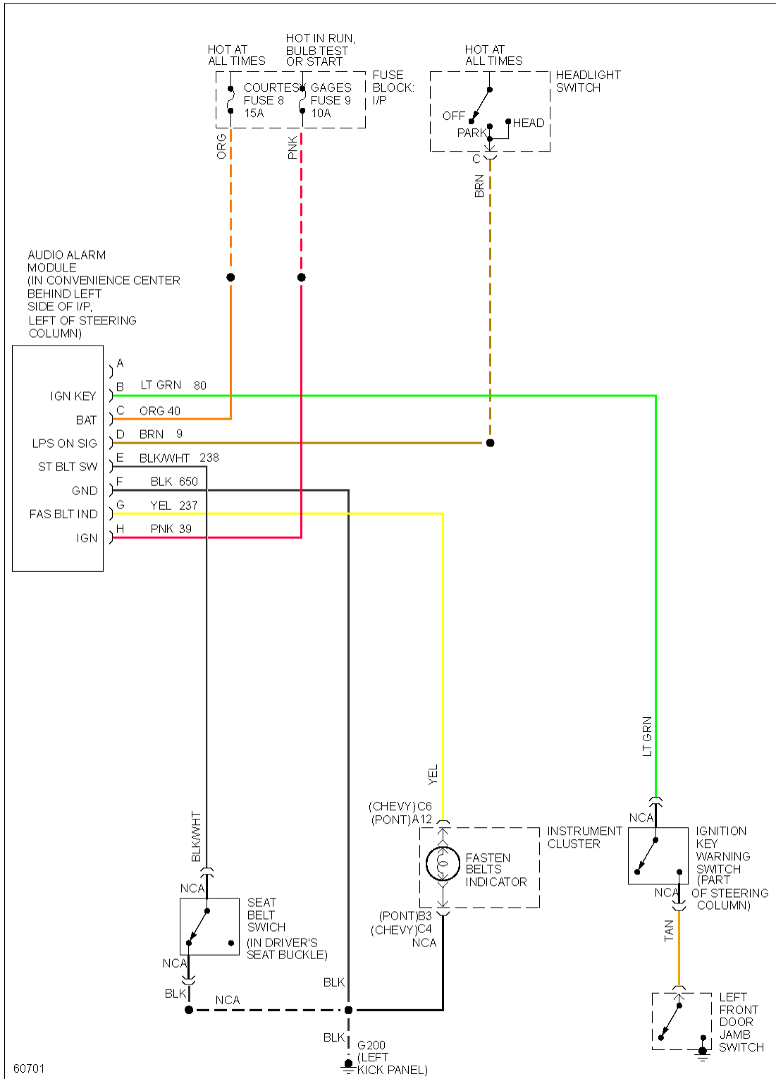
Fig. 46: Warning System Circuits
