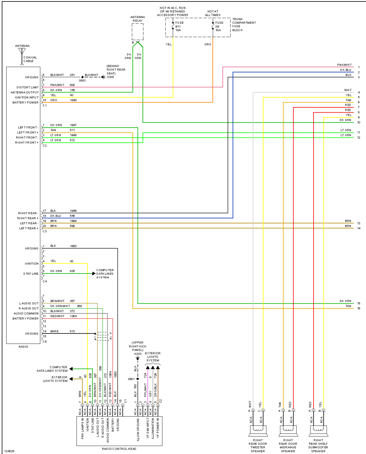
Fig. 47: Radio Circuits, W/ Amplifier (1 of 2)
