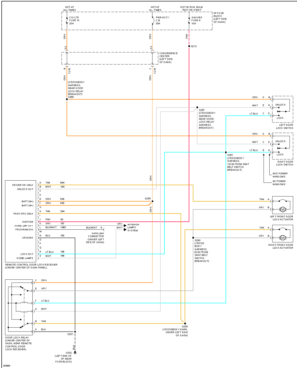
Fig. 61: Keyless Entry Circuit, W/O Crew Cab
