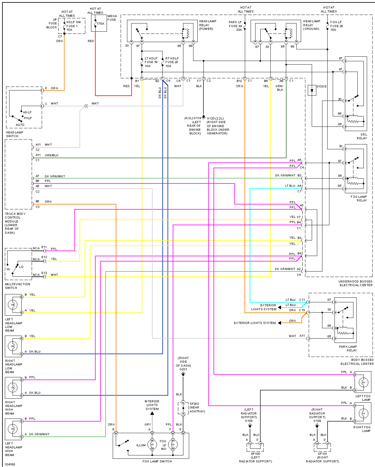
Fig. 21: Headlamps/Fog Lamps Circuit
