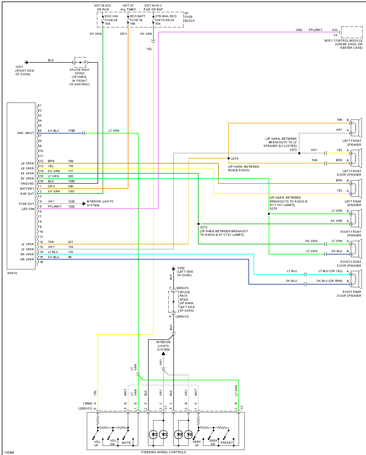
Fig. 42: Radio Circuits, W/O Amplifier
