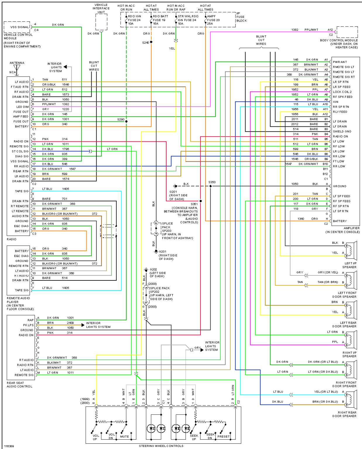
Fig. 45: Radio Circuits
