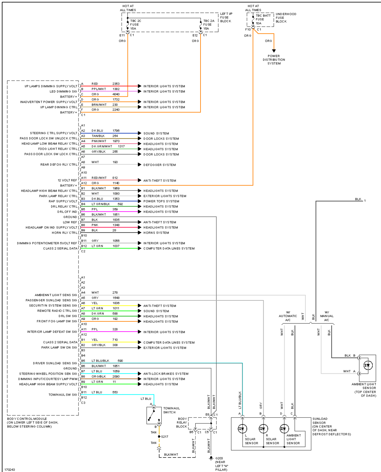
Fig. 15: Body Control Modules Circuit (1 of 2)
