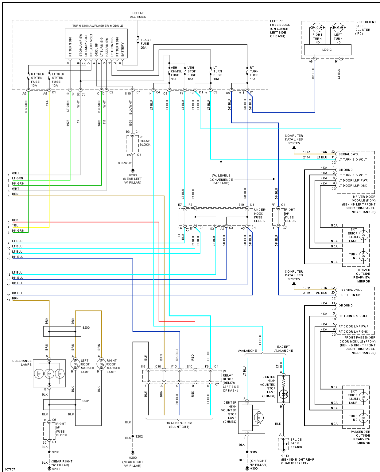
Fig. 47: Exterior Lamps Circuit (3 of 3)
