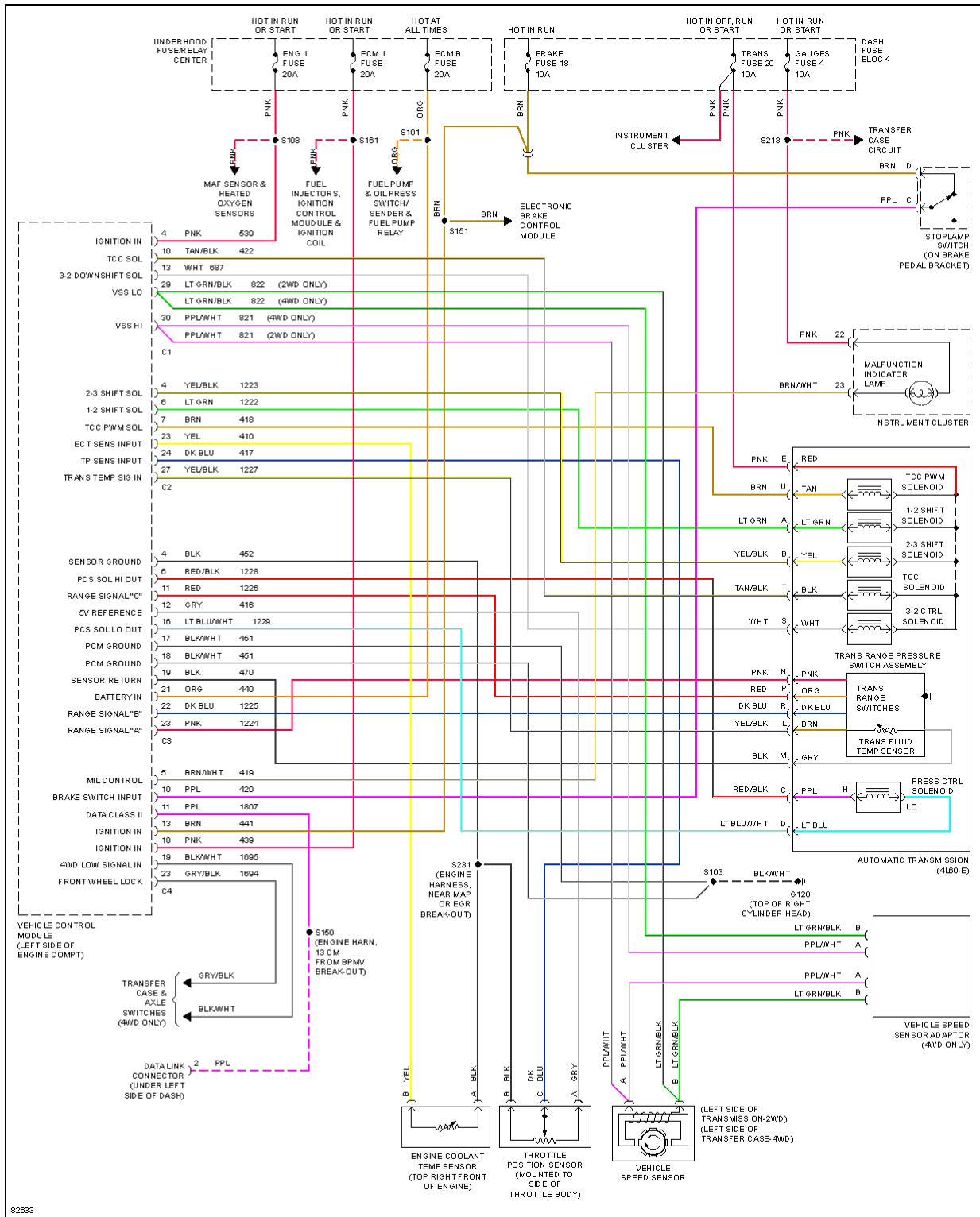
Fig. 80: 5.7L (VIN R), Transmission Circuit, 4L60-E
