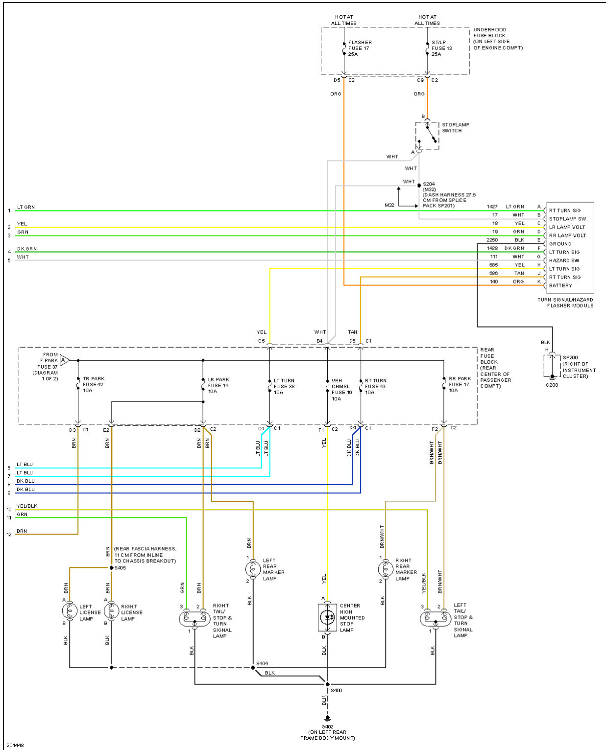
Fig. 20: Exterior Lamps Circuit (2 of 2)
